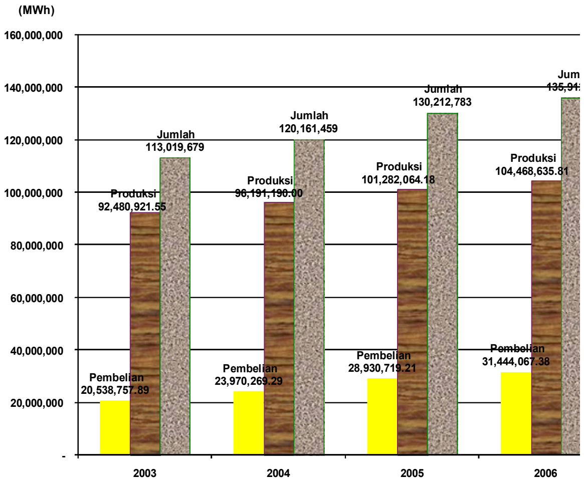
Produksi dan Pembelian Tenaga Listrik PLN (2003 - 2007) PLN's Electricity Production By Type Of Power Plant
