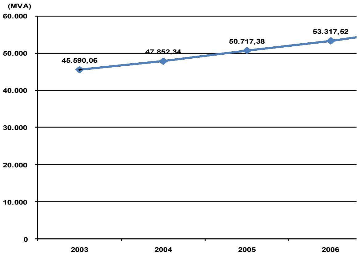
Jumlah Daya Tersambung (2003 - 2007) Number of Power Connected
